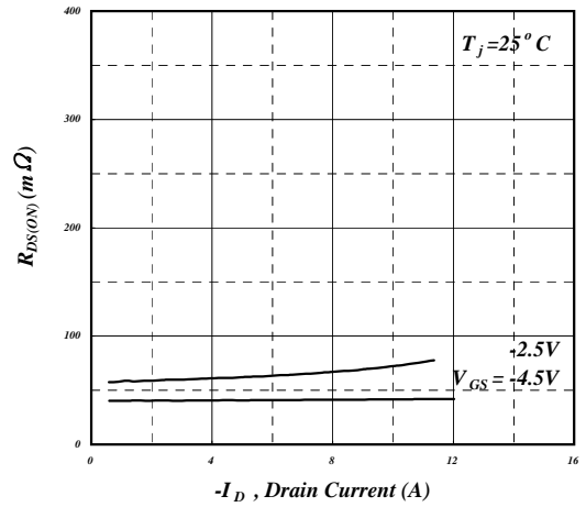
Fig 15. Typ. Drain-Source on State Resistance
