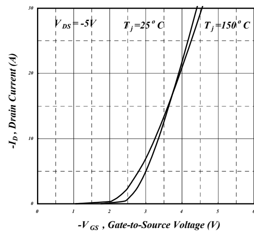
Fig 16. Transfer Characteristics
