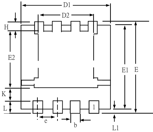
BACKSIDE VIEW
