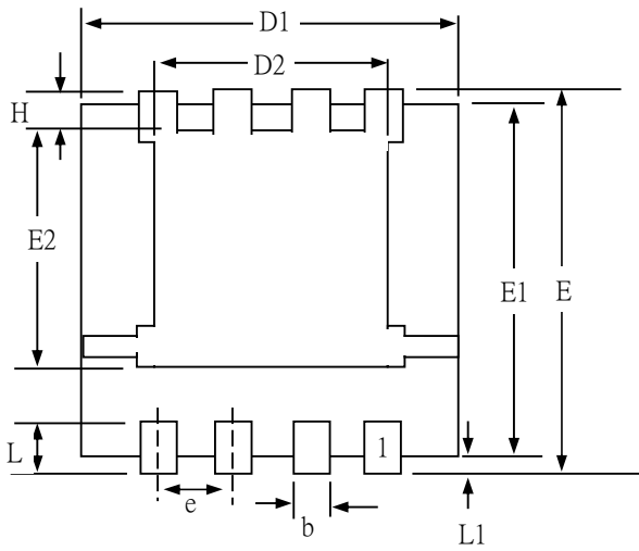
BACKSIDE VIEW
