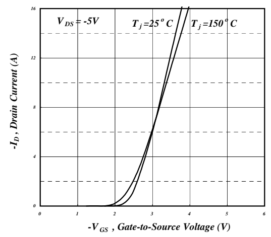
Fig 12. Transfer Characteristics
