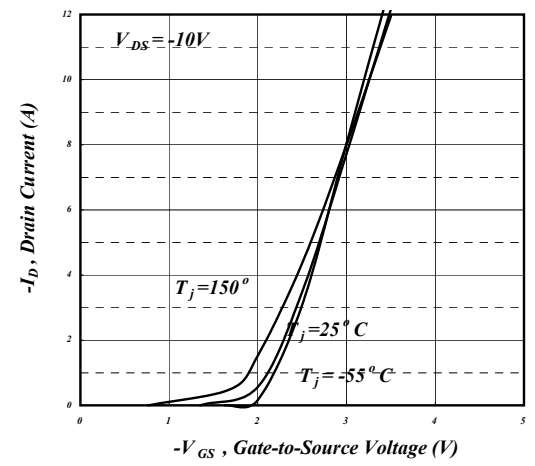
Fig 12. Transfer Characteristics
