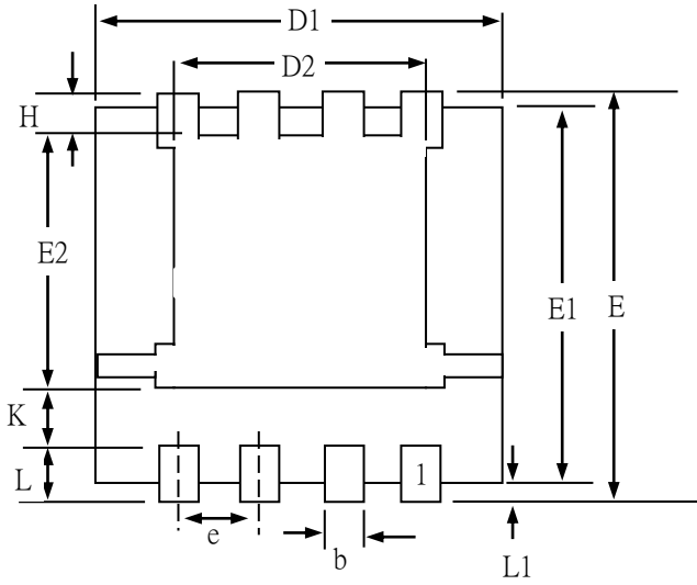
BACKSIDE VIEW
