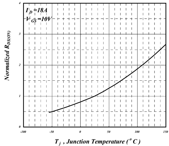
Fig 4. Normalized On-Resistance
