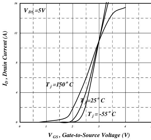
Fig 15. Transfer Characteristics
